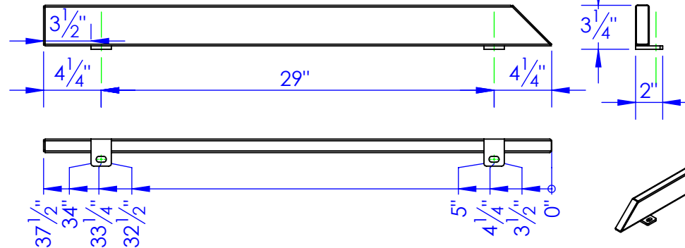
SUB-SIDERAIL 3299 RH SIDE RAIL 3300 RIGHT HAND
