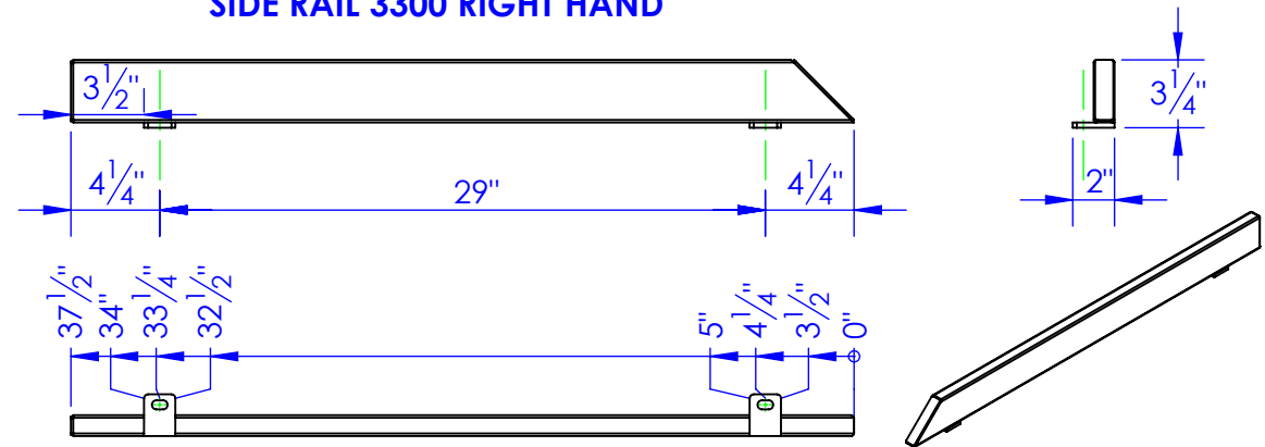
SUB-SIDERAIL 3299 RH SIDE RAIL 3300 RIGHT HAND
